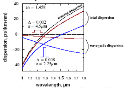
Figure 1.26 Dispersion of two types step-index fibres with the same V-values 1.4 Dispersion of optical fibres C. Dispersion controlled fibres
