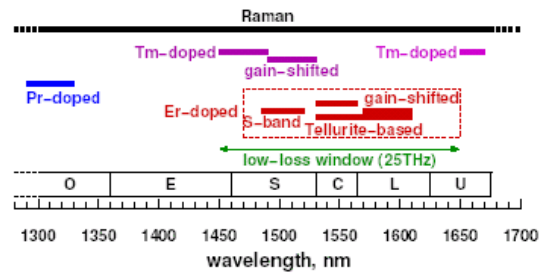
Figure 8.40 Wavelength bands of various optical amplifiers
