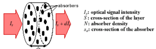
Figure 4.14 Optical intensity evolution in a thin layer containing absorbers
